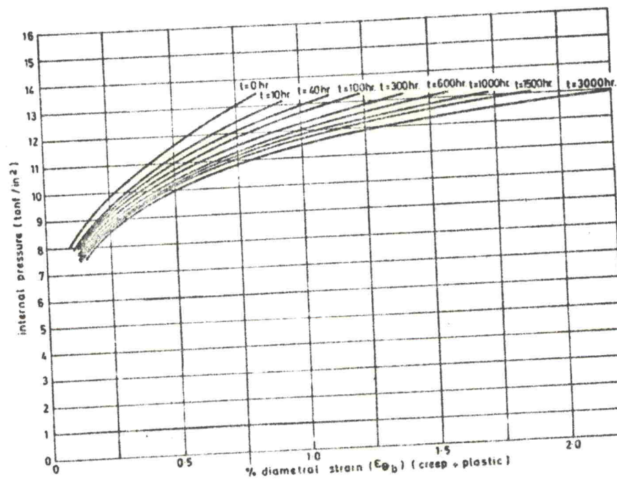
FIG. 15 ISOCHRONOUS PRESSURE-EXPANSION CURVES PREDICTED BY TORSION CREEP DATA (0.18 PERCENT CARBON STEEL AT 400°C)
